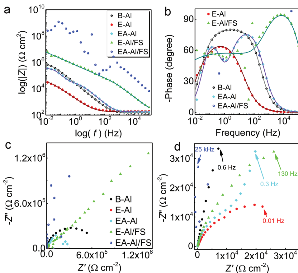
Figure 8. Electrochemical impedance spectroscopy measurements of the B-Al, E-Al, EA-Al, E-Al/FS, EA-Al, and EA-Al/FS surfaces. Bode plots of a) impedance modulus |Z| , b) phase angle versus frequency, c) Nyquist plots, and d) their zoom-in view in the high-frequency region. The solid lines in (a-b) represent the fitted equivalent circuit impedance. The EIS data were measured in an aqueous borate electrolyte.
